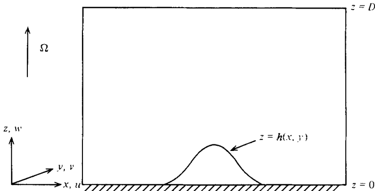
FIGURE 1. Schematic diagram of domain of integration.
