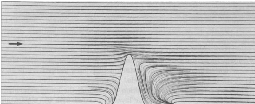
FIGURE 10. Longitudinal (streamwise) section showing velocity directions in the centre-plane for the flow shown in figure 9 (parallel flow).
