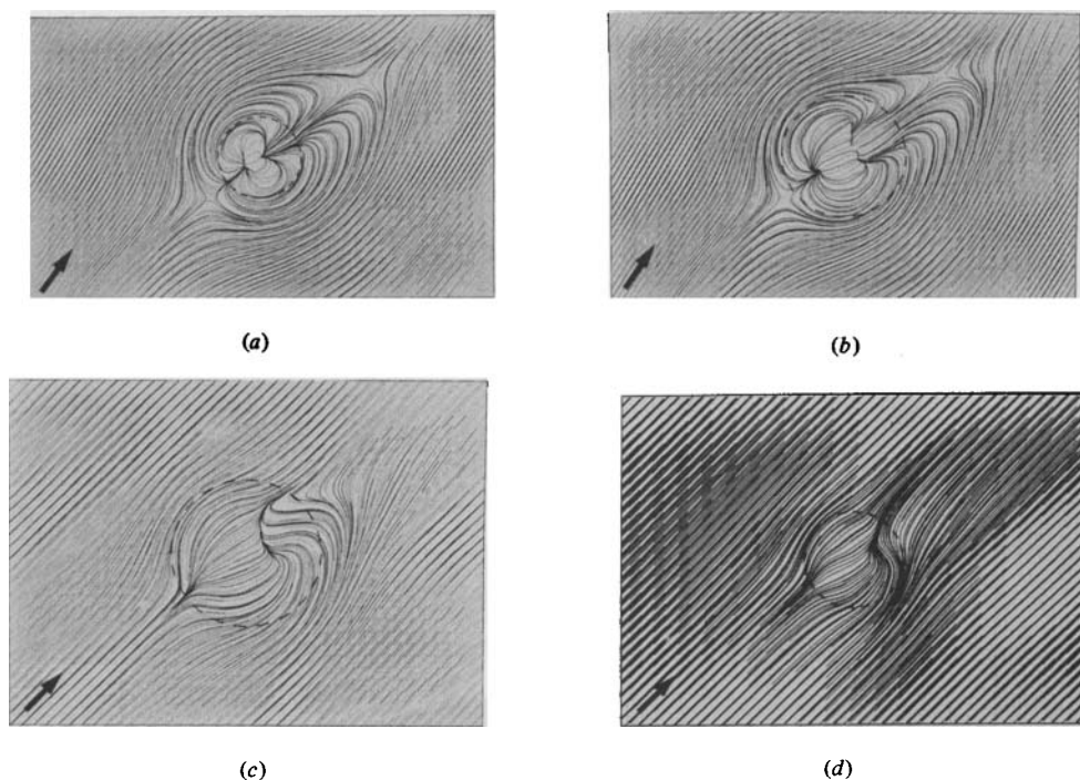
FIGURE 6. Variation of surface stress pattern with h_0/a for Re = 200 ; (a) h_0/a = 3 , (b) h_0/a = 1 , (c) h_0/a = \frac{1}{3} , (d) h_0/a = \frac{1}{6} (Ekman boundary layer).
