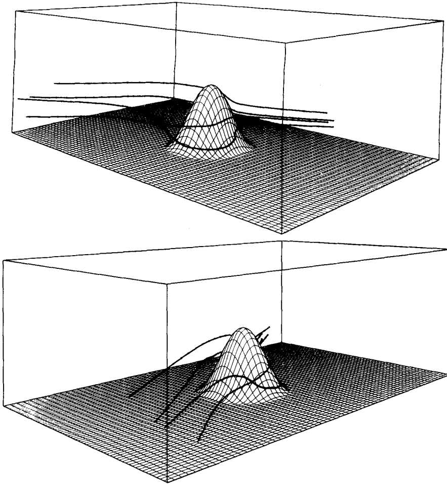
FIGURE 5. Two perspective views of particle trajectories illustrating the upstream separation flow in the case Re = 200 (Ekman boundary layer).
