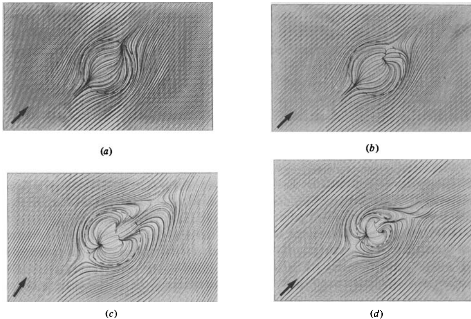
FIGURE 3. Variation of surface stress pattern for Ekman boundary layer flow with Reynolds number; (a) Re = 30 , (b) Re = 60 , (c) Re = 200 , (d) Re = 600 .
