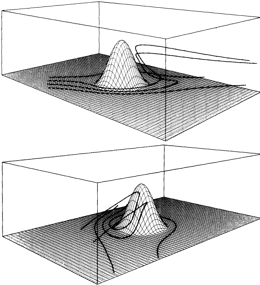
FIGURE 4. Two perspective views of particle trajectories illustrating the rear separation flow in the case Re = 200 (Ekman boundary layer).
