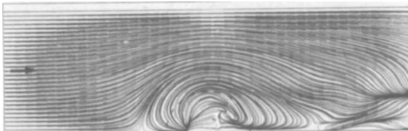
FIGURE 12. Surface stress pattern for parallel flow integration with Re = 300 , h_0/\delta = 2 , h_0/a = 1 .
