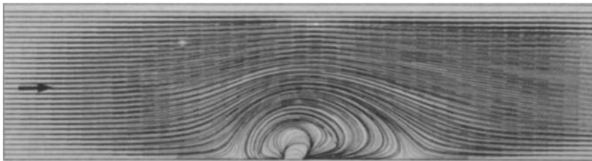
FIGURE 9. Surface stress pattern for parallel flow integration with Re = 200, h_0/\delta = 1 and h_0/a = 3 .
