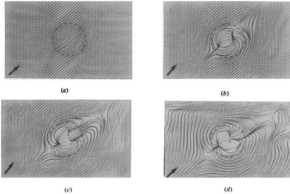
FIGURE 8. Variation of surface stress pattern with h_0/\delta ; (a) h_0/\delta = \frac{1}{4} , (b) h_0/\delta = \frac{1}{2} , (c) h_0/\delta = 1 , (d) h_0/\delta = 2 . The effective Reynolds numbers (see text) are R_h = 6, 24, 100, and 300 respectively (Ekman boundary layer).
