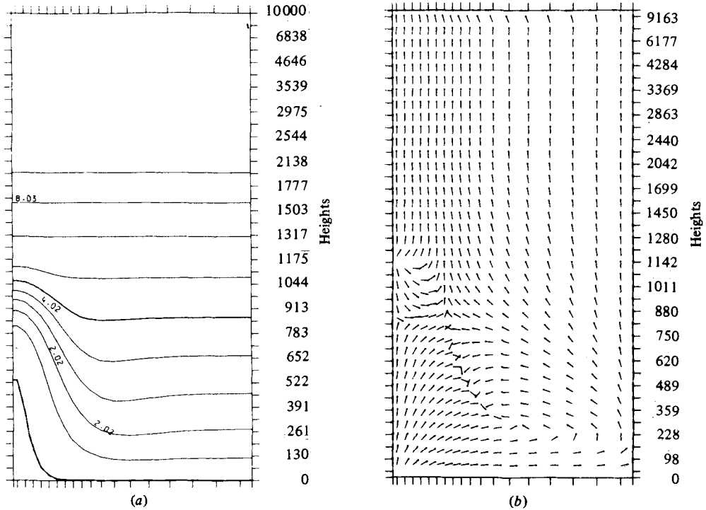
FIGURE 11. Transverse sections taken at the downstream extremity of the obstacle for the flow shown in figure 9 (parallel flow). (a) shows contours of the streamwise velocity component and (b) secondary flow directions. The velocity contour values refer to a dimensionless free stream speed of 10. The vertical scale is plotted with a uniform grid spacing; the actual grid-point coordinates are indicated by the arbitrary height scale on which h_0 has value 1000.
