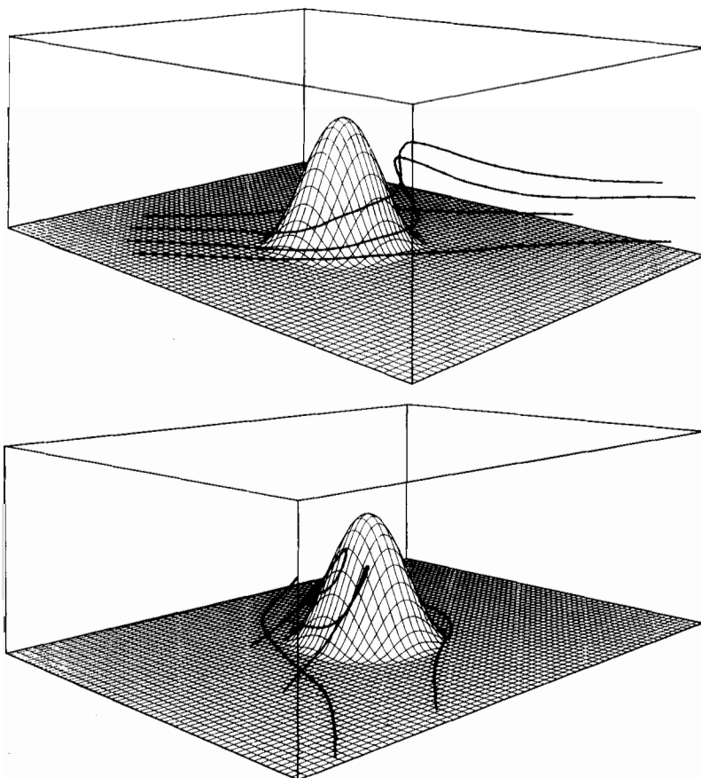
FIGURE 7. Two perspective views of particle trajectories illustrating the rear separation flow in the case Re = 200 , h_0/a = \frac{1}{3} (Ekman boundary layer).
