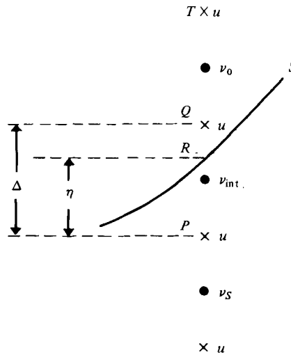
FIGURE 2. Illustrating the intersection of the curved boundary and a line of grid points.
