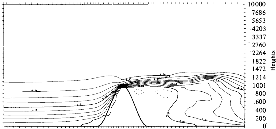
FIGURE 15. Longitudinal (streamwise) section showing contours of the streamwise velocity component for the parallel flow shown in figure 12.
