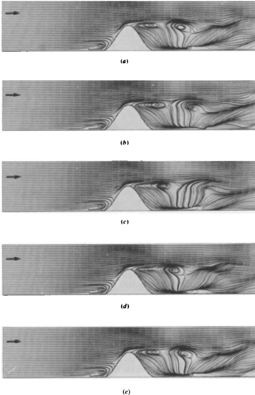
FIGURE 14. Longitudinal (streamwise) sections showing velocity directions in the centre-plane for the parallel flow shown in figure 12 at different times. The dimensionless times, in units of a/U_0 , are (a) 68.9, (b) 70.5, (c) 72.1, (d) 73.7, (e) 75.3.
