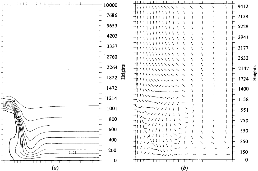
FIGURE 13. Transverse sections taken at the downstream extremity of the obstacle for the parallel flow shown in figure 12. (a) shows contours of the streamwise velocity component and (b) secondary flow directions. The arbitrary scales are as with figure 11.
